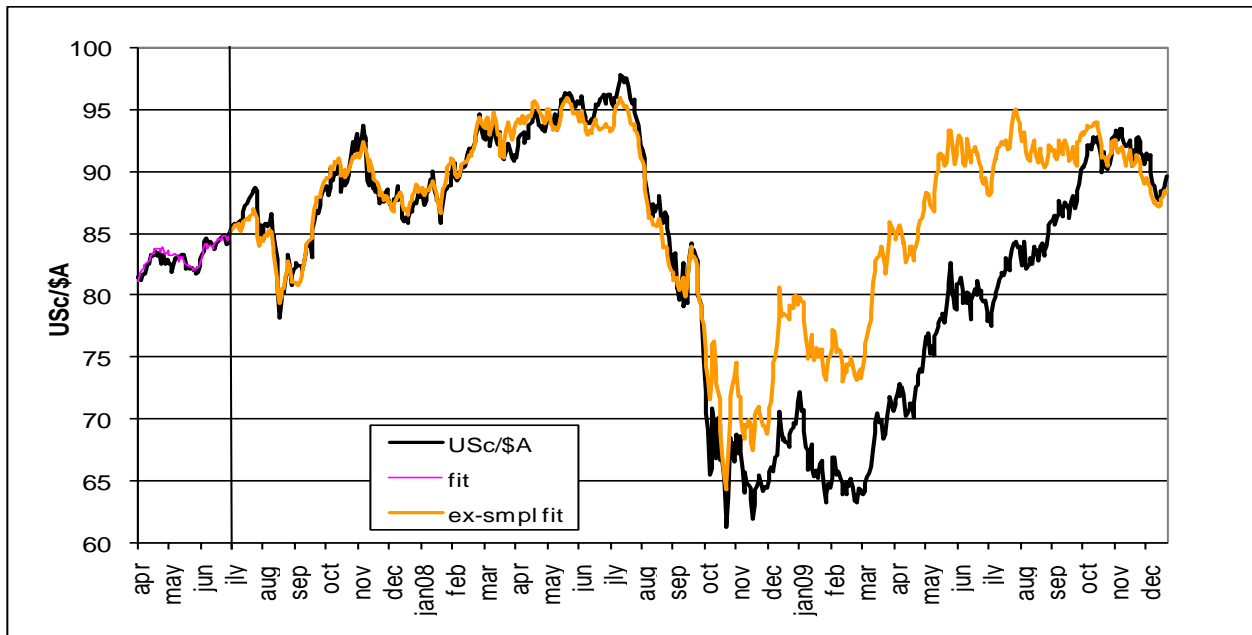
Figure 11 Fit and ex-sample fit of exchange rate equation, 2007 to 2009
